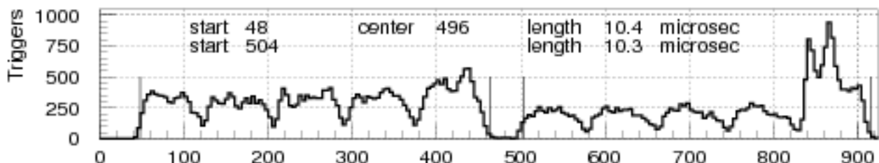
Fig.6 Trigger Time mod. SPS period (1.2 - 2.2 secs) (25ns)
