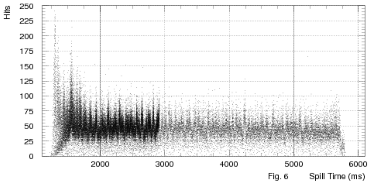
Hits GTK(1) vs Spill Time, Folded Spill Time
