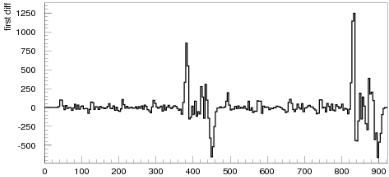
Fig. 9 uncorr. folded time
