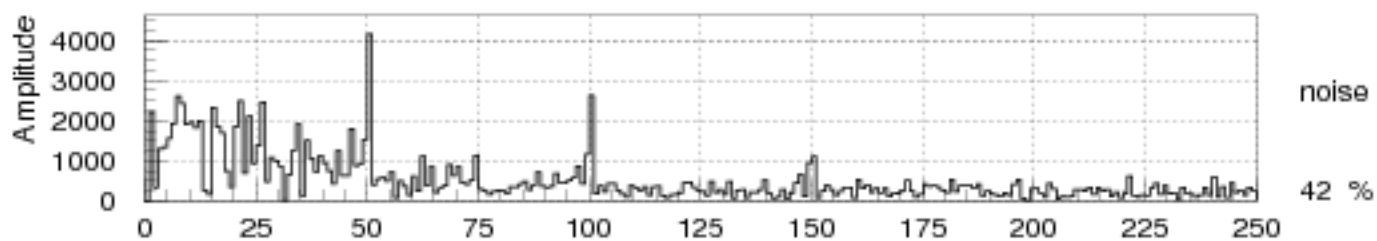
Fig. 3 Frequency (Hz)
