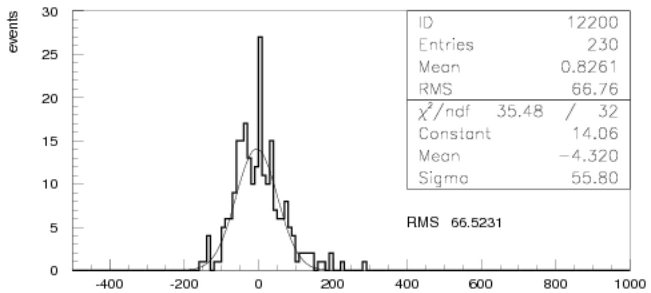
Fig. 10 first diff folded spill time
