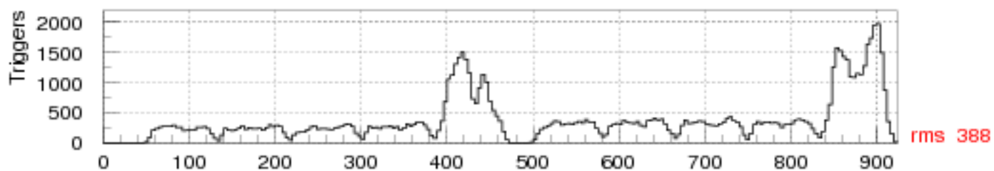
Fig.2 Uncorrected folded spill (1.2 - 2.2 secs)
