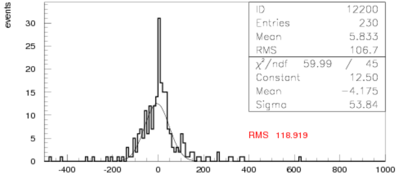
Fig. 10 first diff folded spill time
