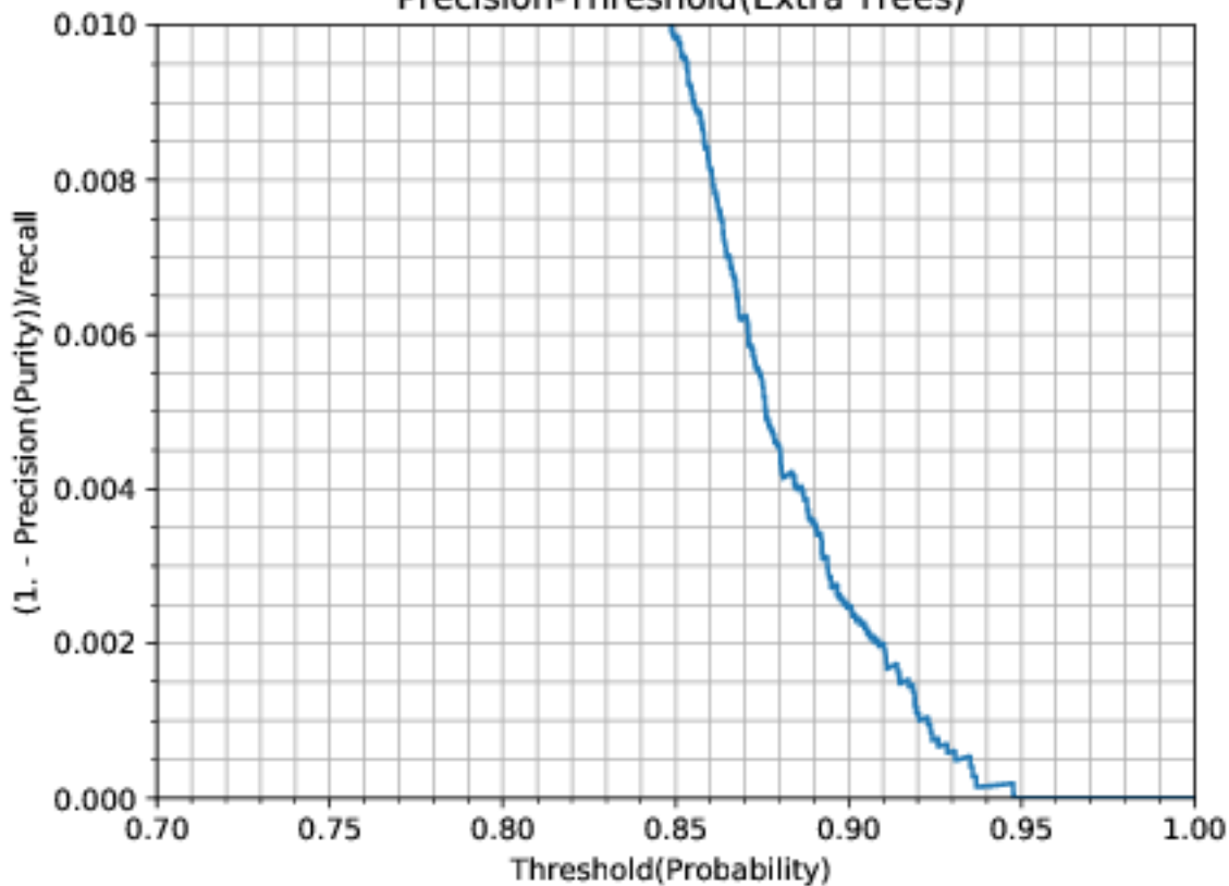
Precision-Threshold(Extra Trees)
