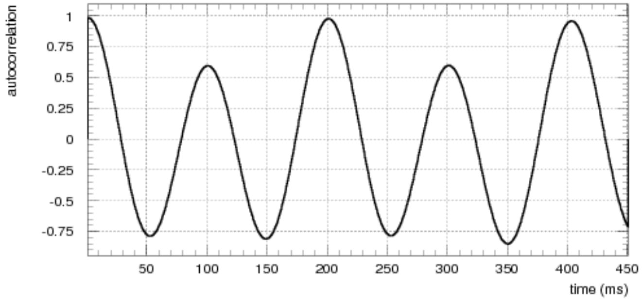
sample autocorrelation
