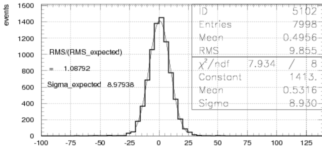
Fig. 4 First difference for events/0.5 ms
