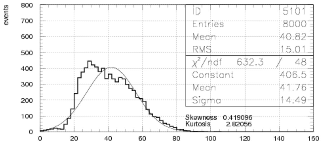
Fig. 2 Spill: distribution of events/0.5 ms
