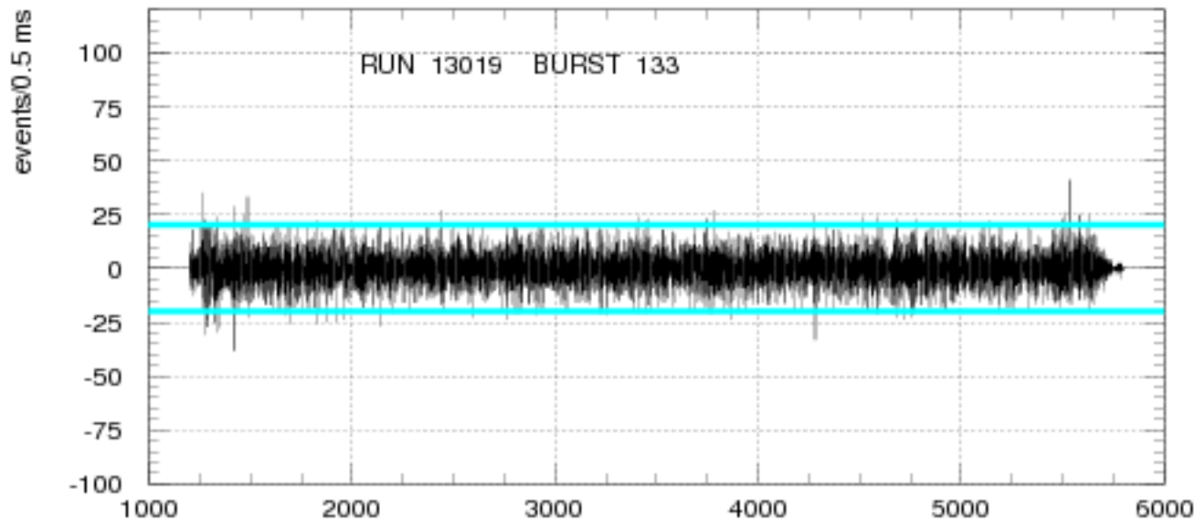
Fig. 3 First difference
