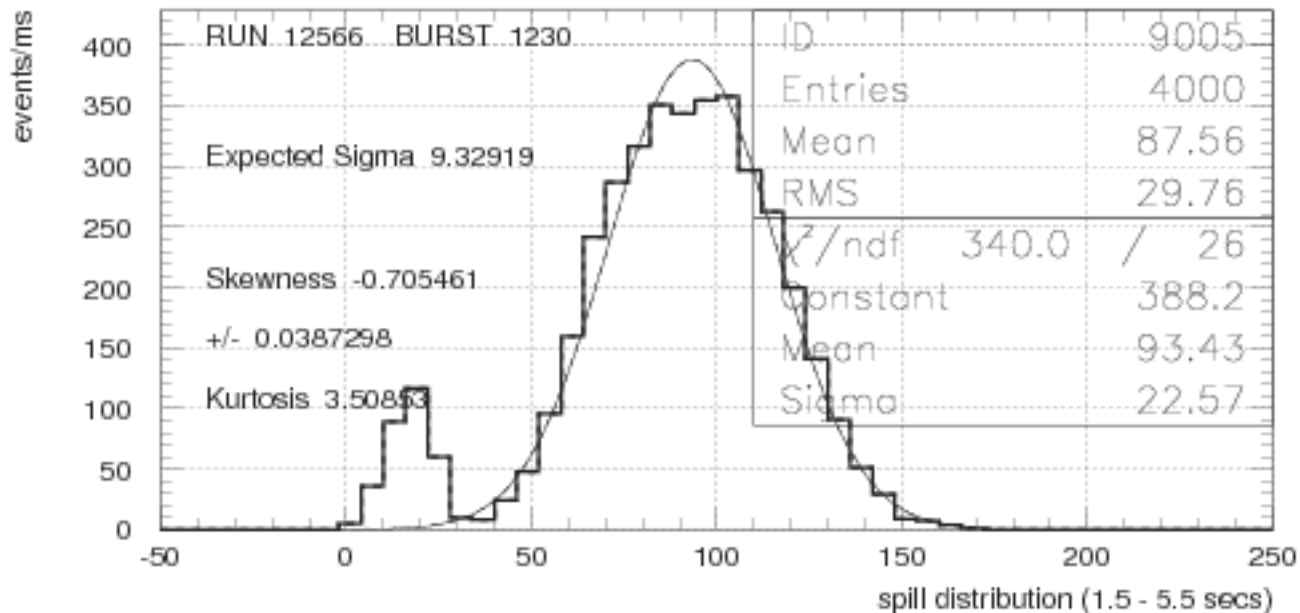
Fig. 3 Spill Distribution
