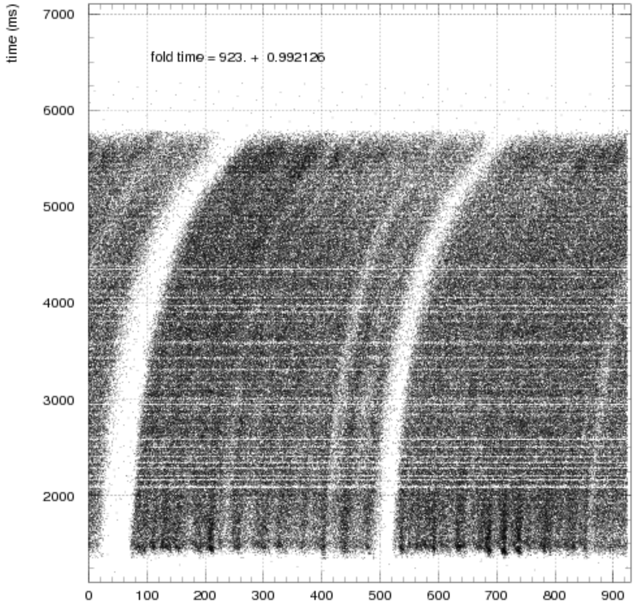
Fig. 2 Folded time/25ns
