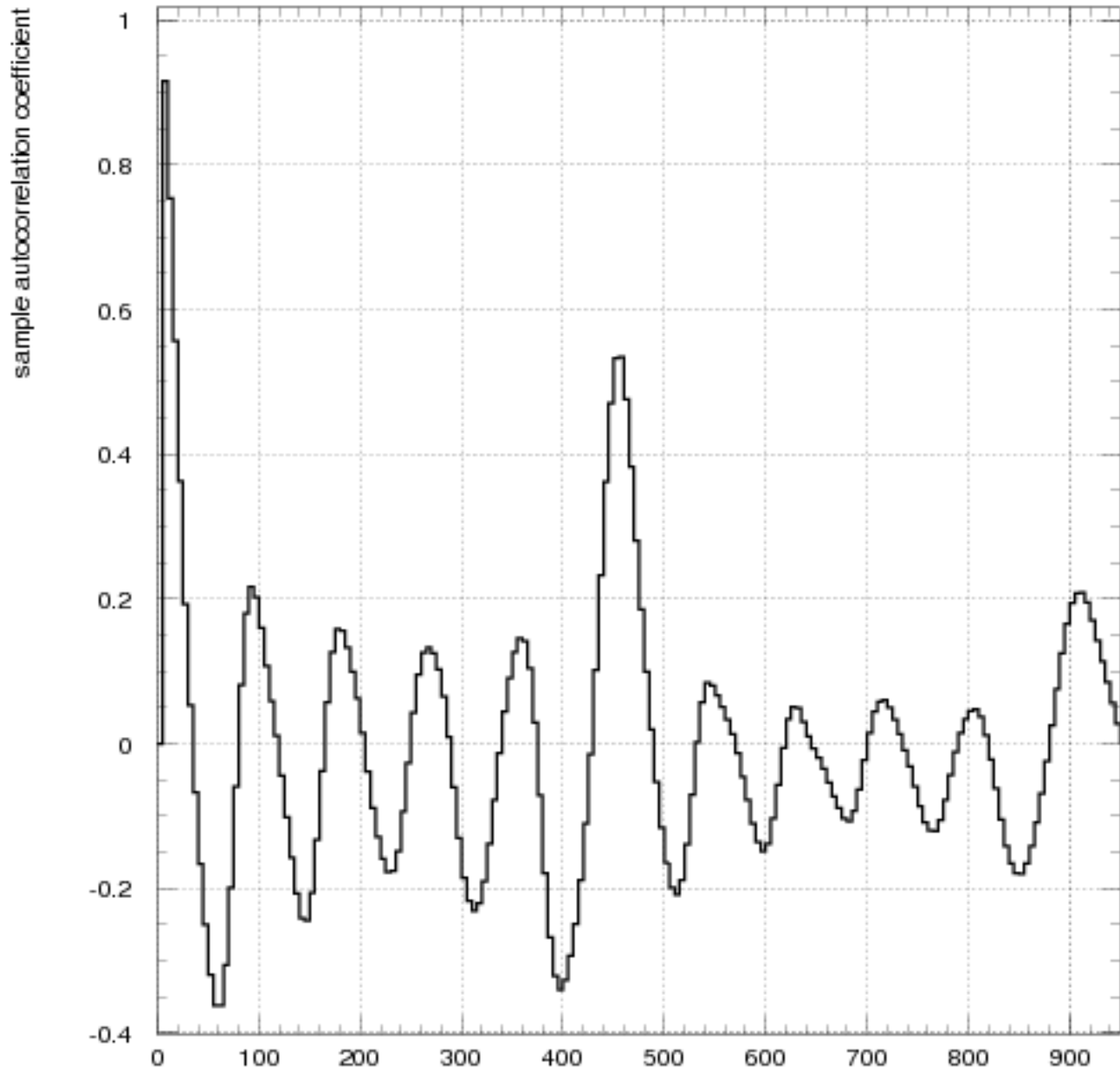
Fig. 5 Time lag (corrected folded time)
