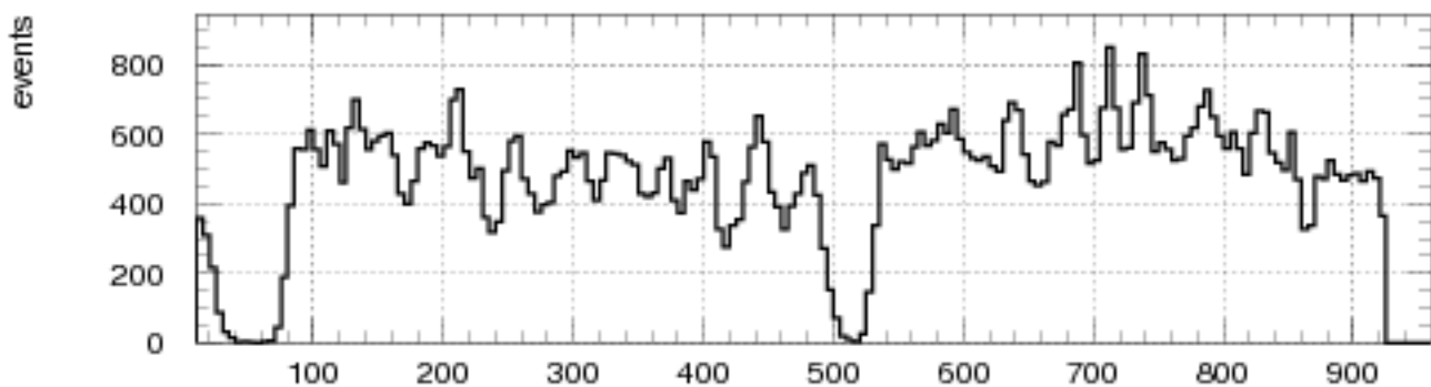
Fig. 4c Uncorrected folded time for 1500-2500 ms spill time
