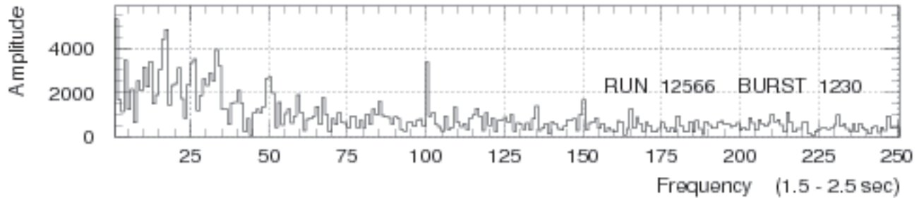
Fig. 2 Modified PERIODOGRAM
